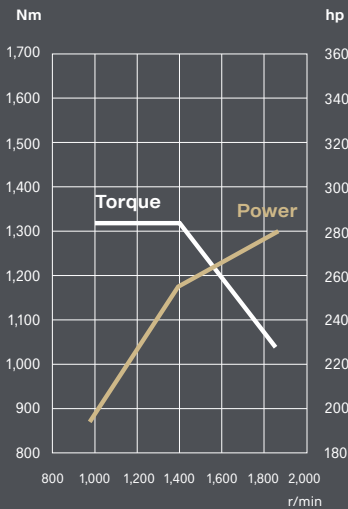
280 hp gas
