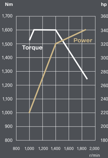
340 hp gas
