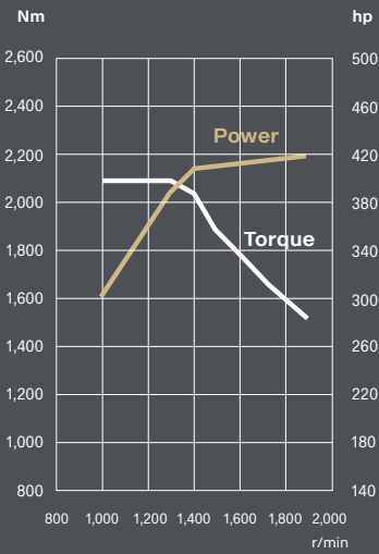
420 hp gas
