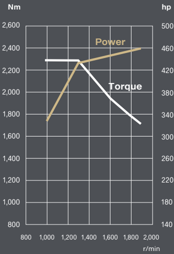
460 hp gas
