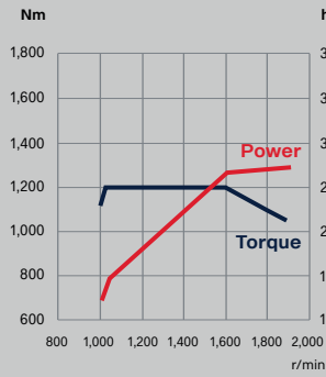
7-litre, 280 hp Biodiesel, HVO, diesel
