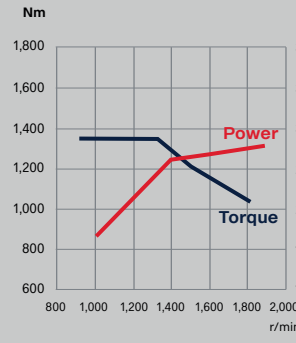
9-litre, 280 hp Biogas, natural gas
