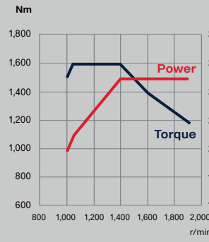
9-litre, 320 hp Biodiesel, HVO, diesel
