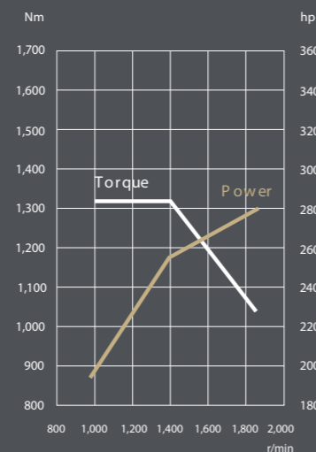
280 hp gas
