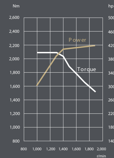
420 hp gas
