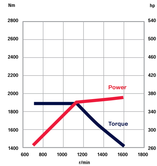
13-litre, 370 hp HVO, diesel
