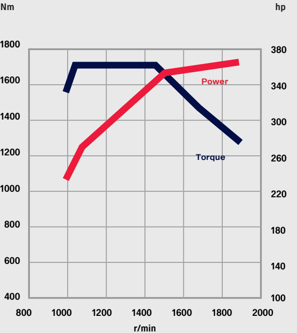
9-litre, 360 hp Biodiesel (B100%), HVO (B7%), diesel
