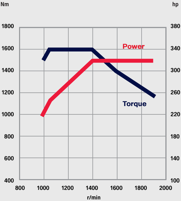
9-litre, 320 hp Biodiesel (B100%), HVO (B7%), diesel
