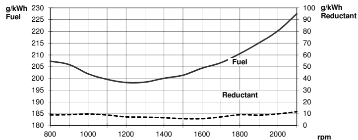
Spec fuel and reductant consumption
