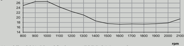
Reductant consumption
