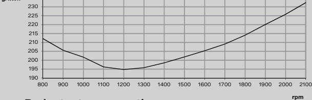
Reductant consumption
