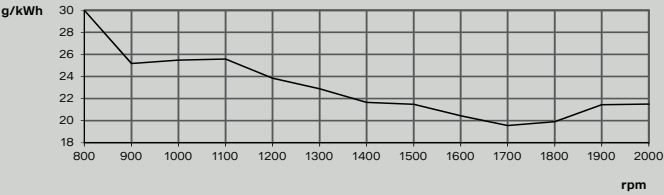
Reductant consumption
