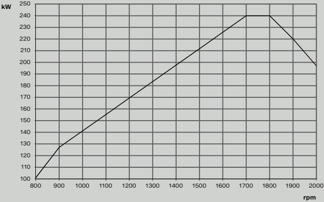
Power
