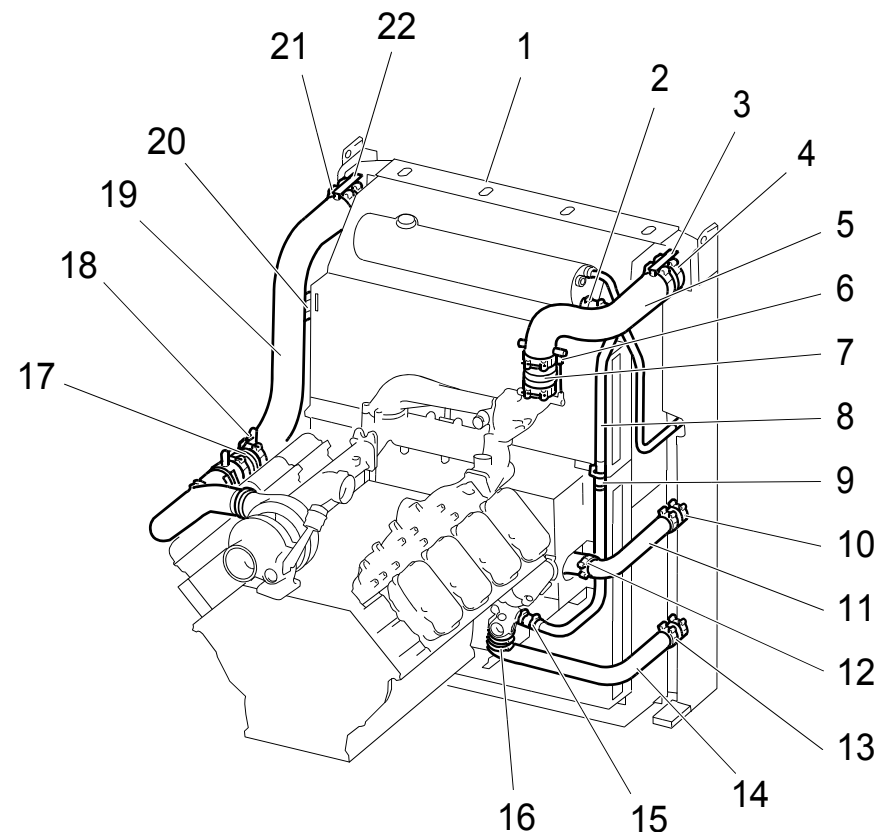
1.5 m 2 radiator for the DC16
