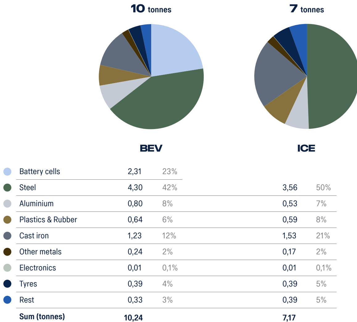
Figure 3. Material composition of the two vehicles.
