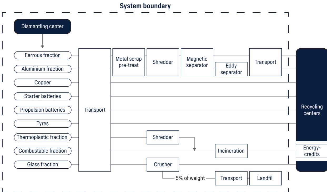
Figure 4. End-of-life schematic overview.
