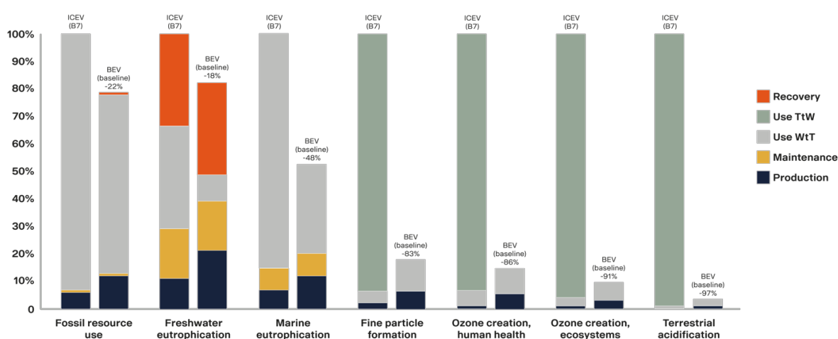
Figure 9. BEV reduction potential for other impact categories. BEV reduction values presented in relation to ICEV emissions.
