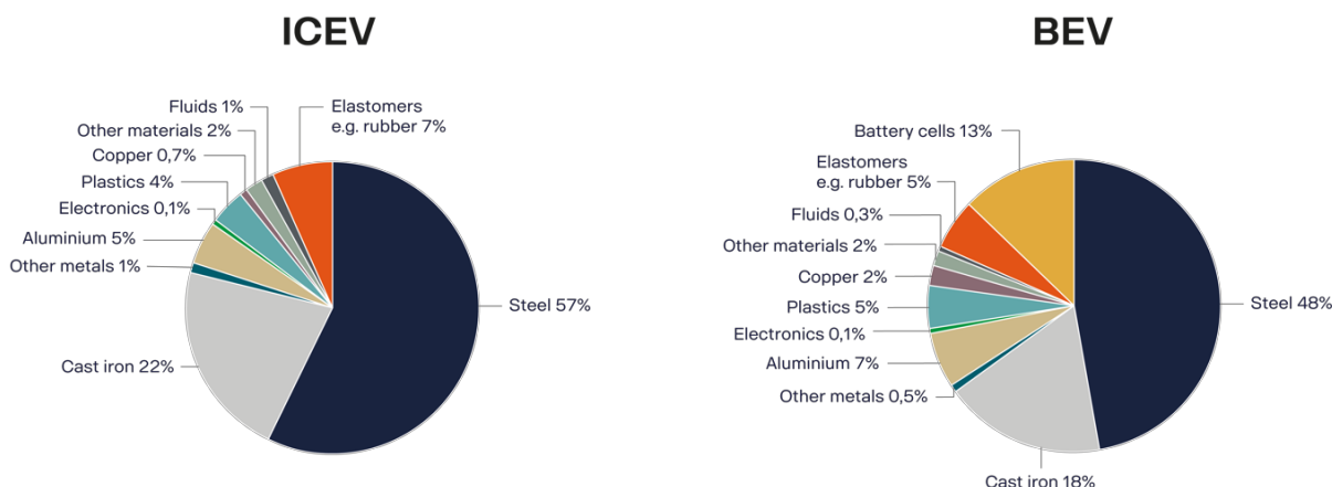
Figure 2. Material composition. Material categories expressed in percent of total vehicle weight.
