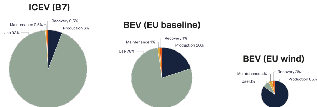
Figure 5. Share from each life cycle phase in % of total life cycle GHG emissions. The sizes of the circles are proportional to total life cycle GHG emissions.
