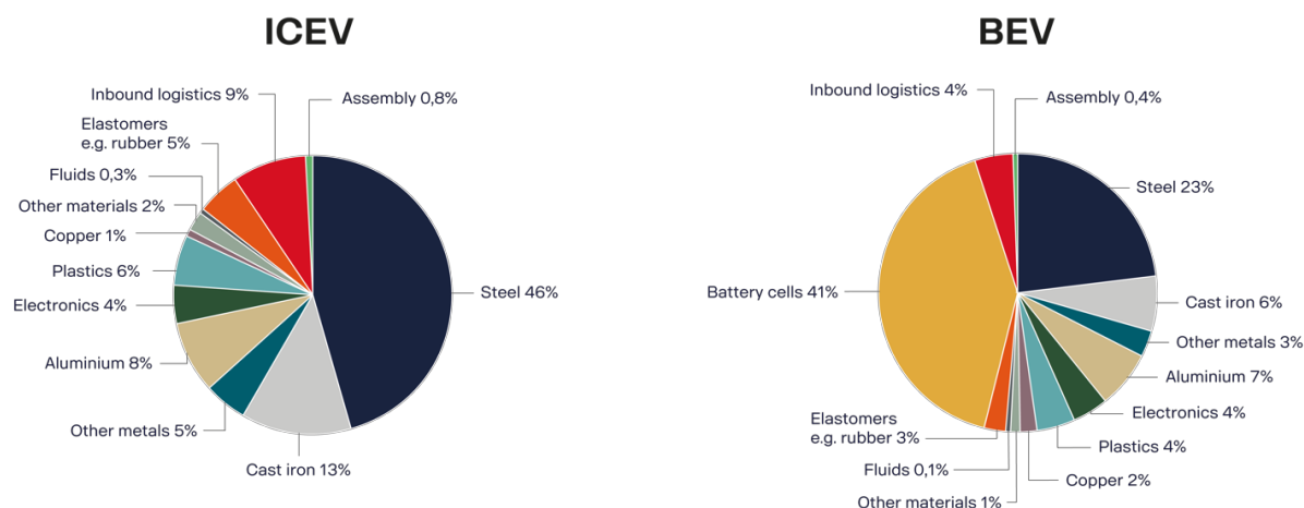
Figure 6. GHG emissions from different material categories in % of total emissions from production phase.
