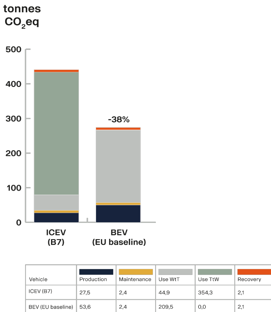
Figure 3. Total life cycle GHG emissions presented as tonnes of CO 2 eq per life cycle phase. The use phase is divided in well-to-tank and tank-to-wheel.
