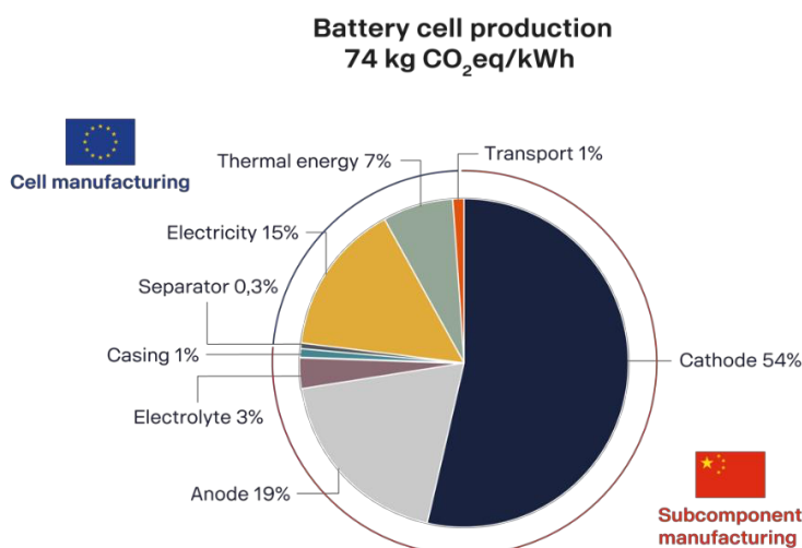
Figure 7. GHG emissions from different steps in battery cell production in % of total impact per kWh installed capacity.
